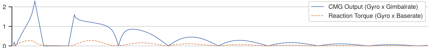
Gimbal Torque Components Magnitude [Nm]
